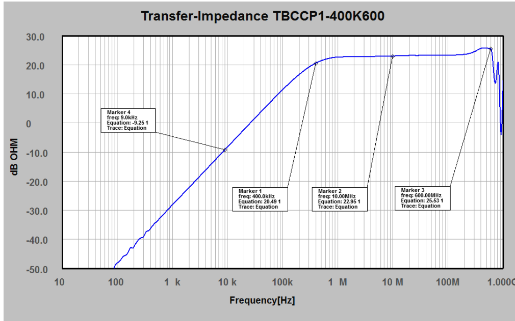
Figure 1: transfer impedance, 10 Hz – 1 GHz, typical data
