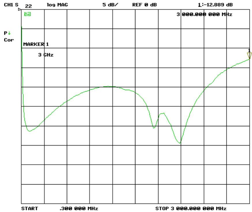
Picture 16 – TBWA1/20dB, output return loss, IS22, 300 kHz – 3 GHz, lin.
